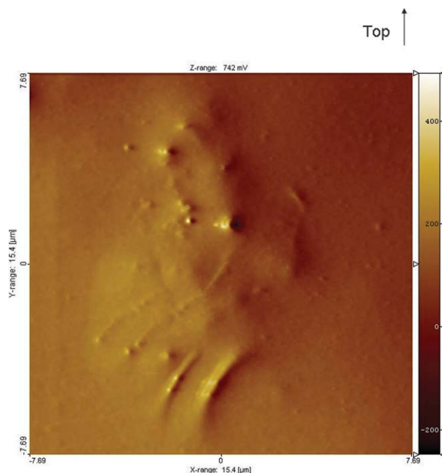
Figure 3 The sheared poly(HEMA)-functionalized multi-wall carbon nanotubes are isolated and evenly spaced with the long axis aligned normal to the direction of shear (left to right). The image is \sim 15 \times 15 \mu\text{m} . [Color figure can be viewed in the online issue, which is available at wileyonlinelibrary.com .]
